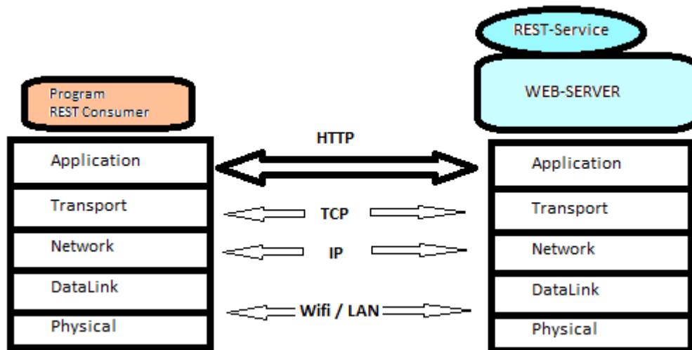
Figur A: Overall Architecture for a REST-Service
